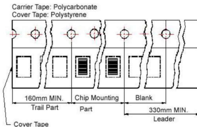
Tape Material
