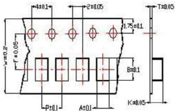
Tape Dimensions
