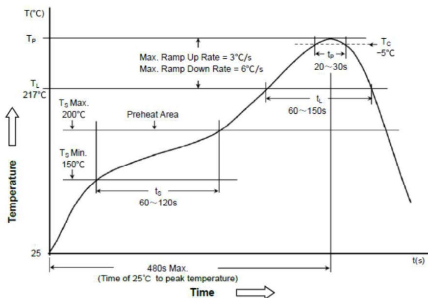
Classification of peak package body temperature (T P )
