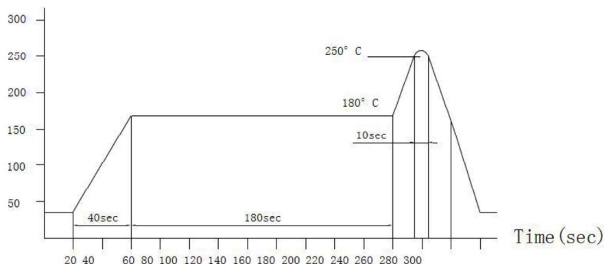
Reflow profile for SMT components
