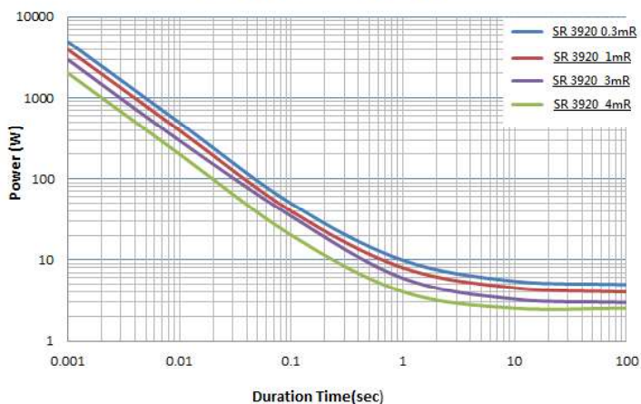
SR 3920 Series Pulsed Power Characteristics
